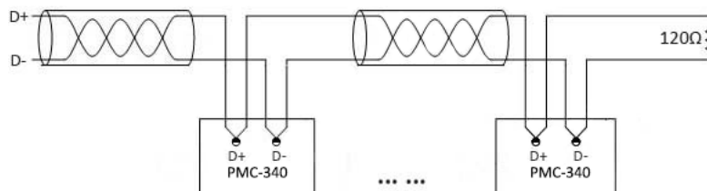
Figure 2-7 RS-485 Connections
