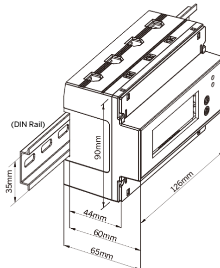
Figure 2-4 Installation
