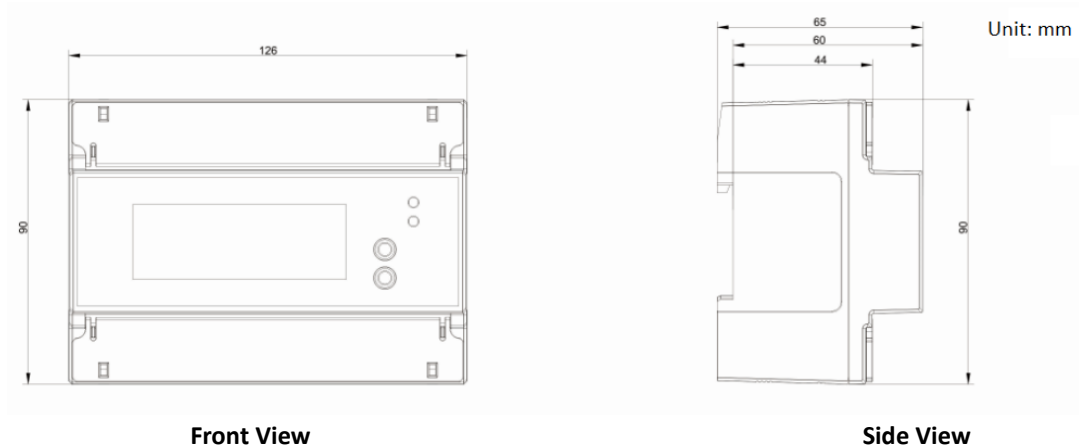
Figure 2-2 Dimensions
