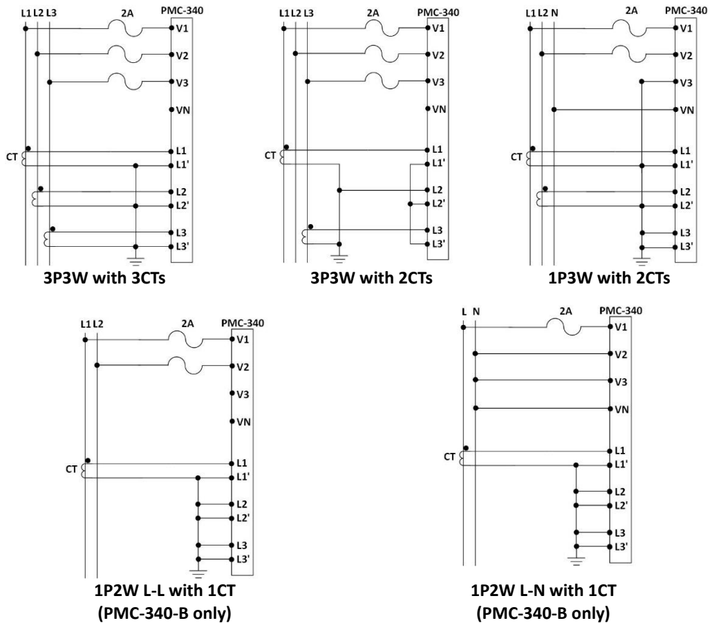
Figure 2-6 5A CT Connect Wiring
