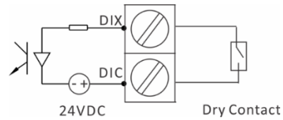
Figure 2-8 DI Connections
