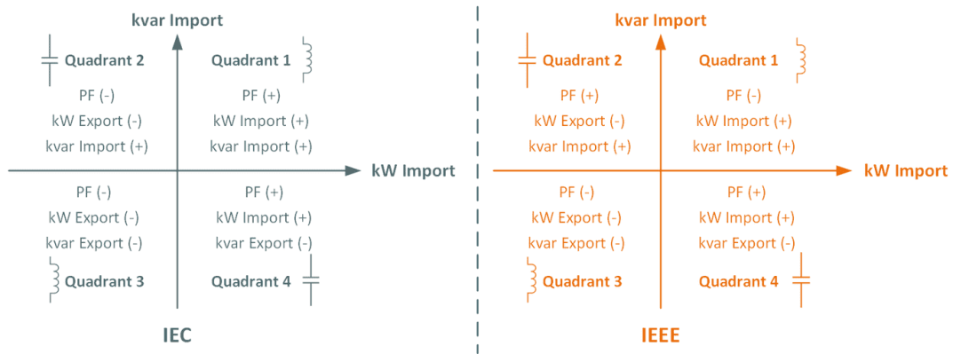
Figure 3-5 PF Convention
