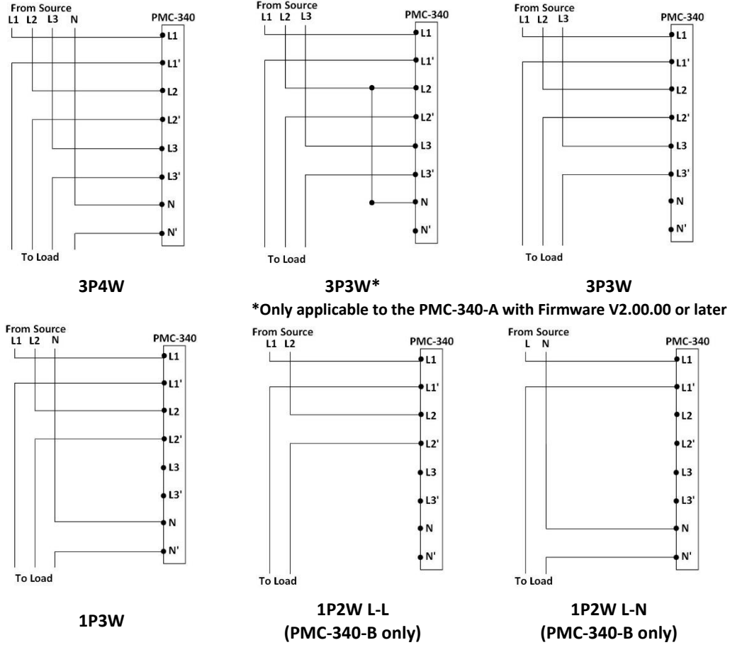
Figure 2-5 100A Direct Connect Wiring
